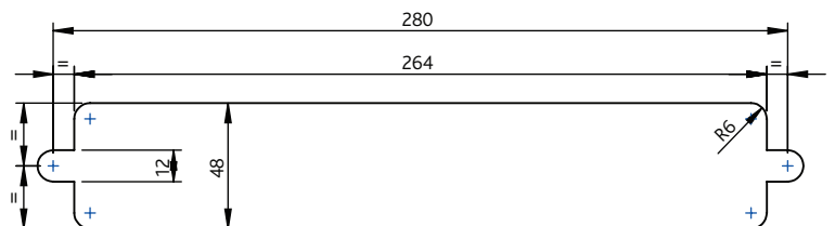
Routing Detail
