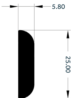
25mm D-Mould
