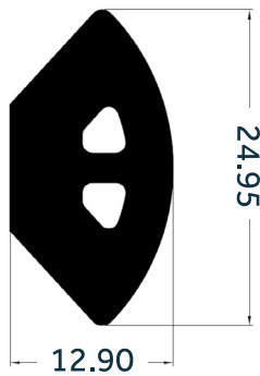
17.5mm Quadrant
